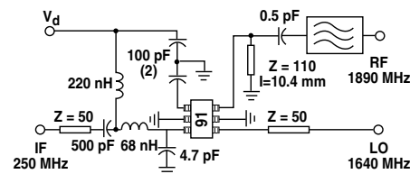
Figure 18. Test Circuit.
