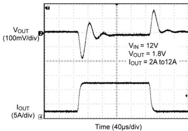
Transient Response
