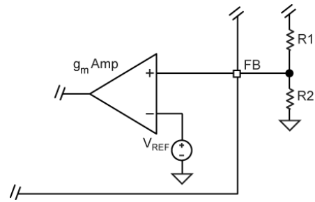
Figure 7. Voltage-Divider Configuration
