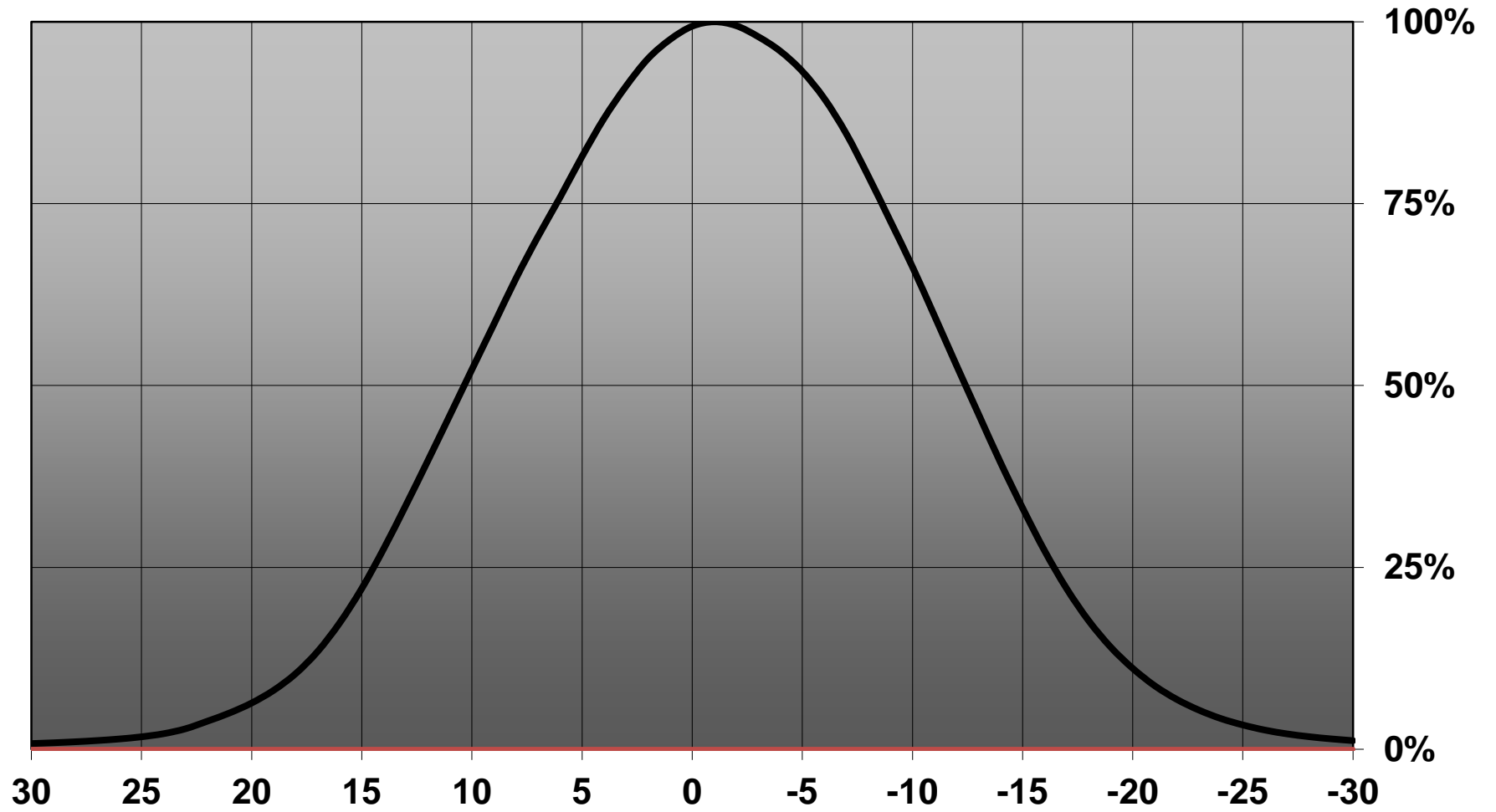
Relative intensity of CA11483_LXP2-M-(XPE2)
