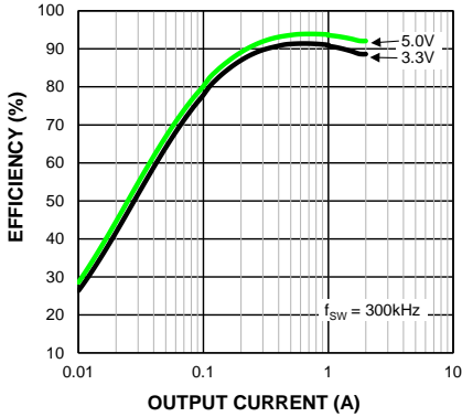
Efficiency (VIN = 12V) vs. Output Current MIC28512-2
