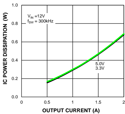
IC Power Dissipation vs. Output Current MIC28512-1
