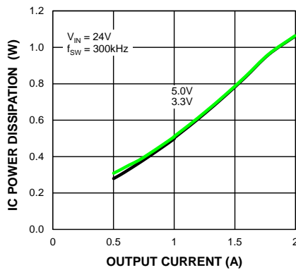
IC Power Dissipation vs. Output Current MIC28512-2
