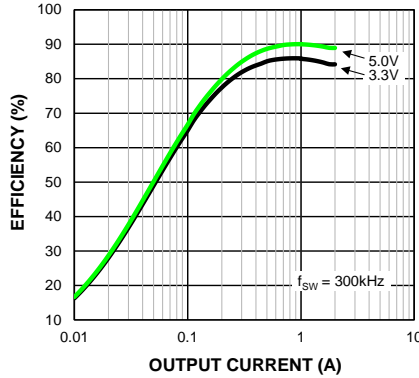
Efficiency (VIN = 24V) vs. Output Current MIC28512-2
