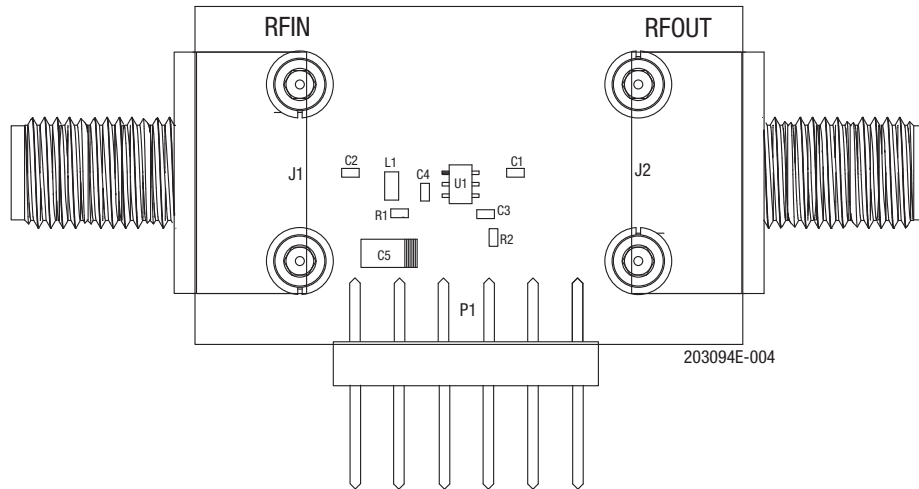
Figure 4. SKY65450-92LF Evaluation Board Assembly Diagram
