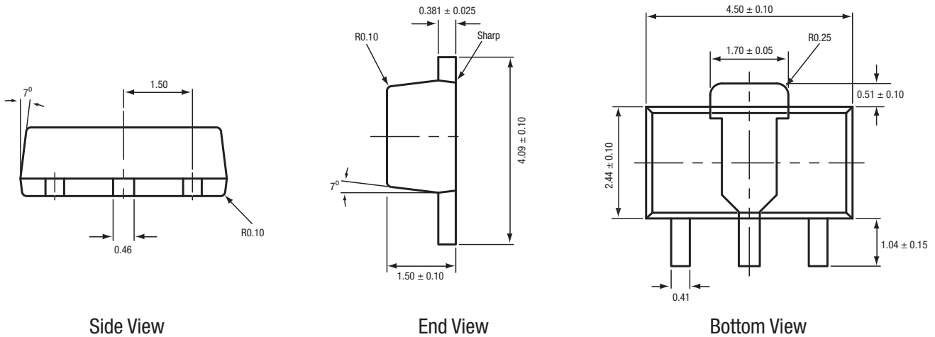
Figure 99. SKY65009 SOT-89 Package Dimensions
