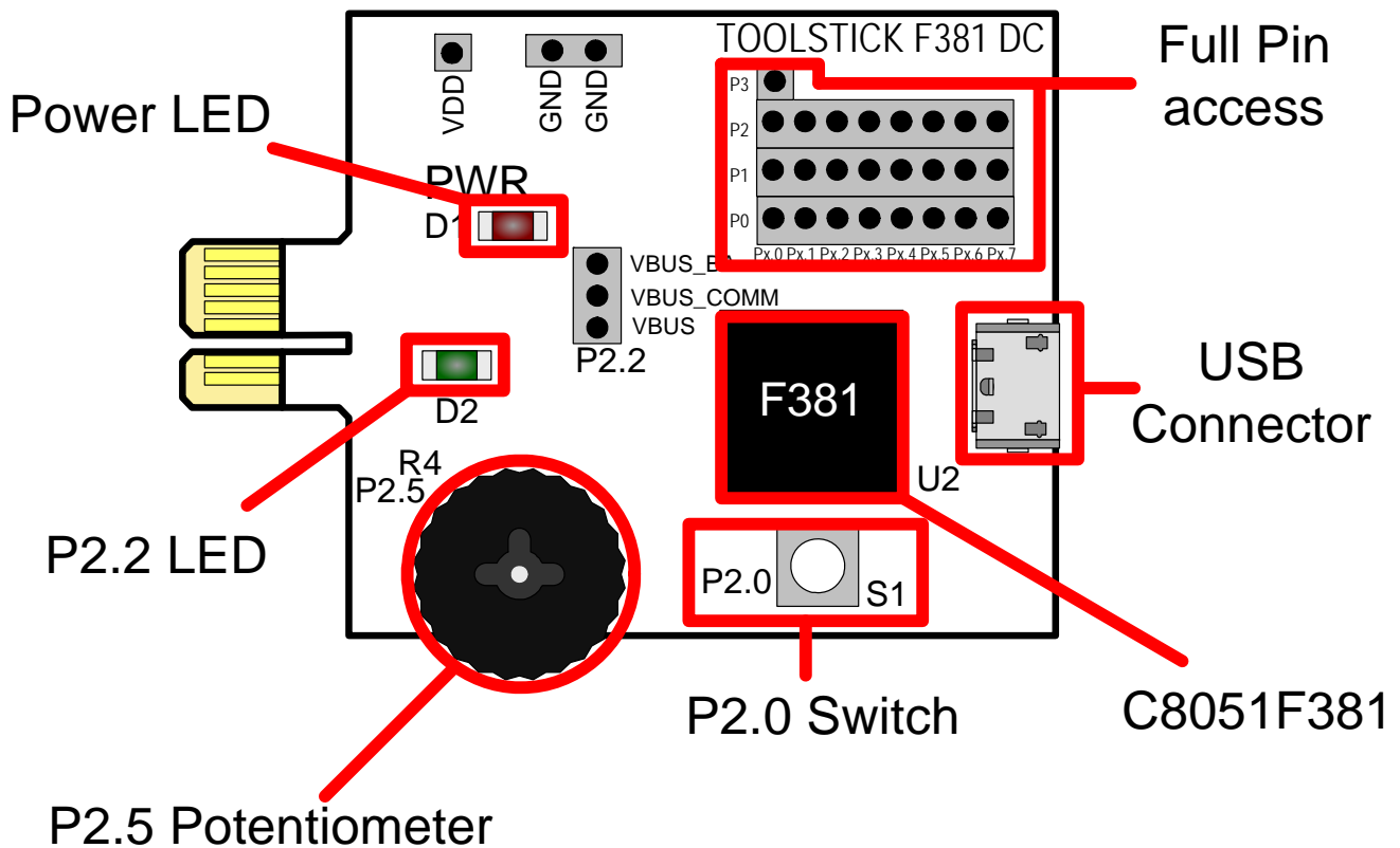
Figure 3. ToolStick C8051F381 Daughter Card
