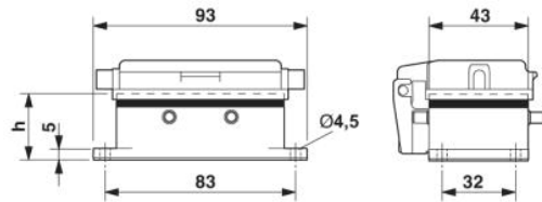
Dimensional drawing
