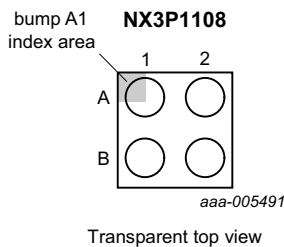
Fig 3. Pin configuration for WLCSP4
