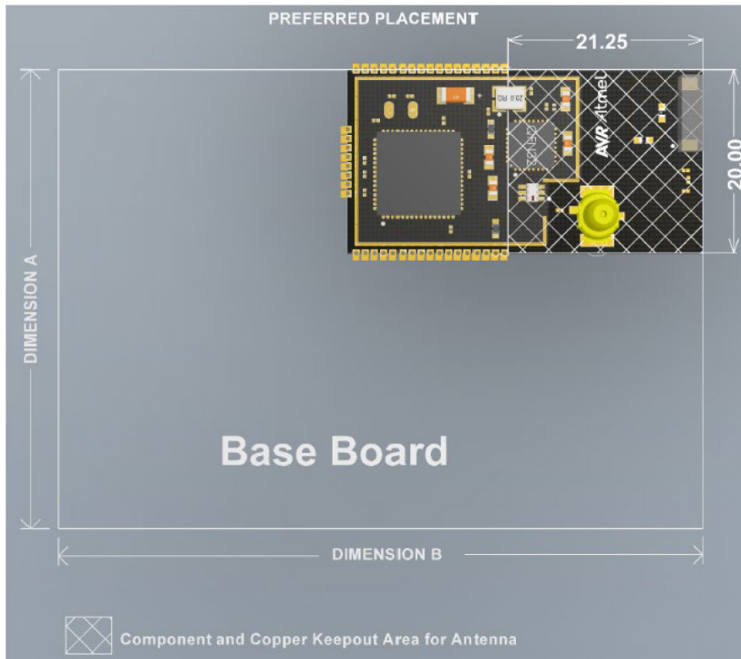
Figure 3-4. ATZB-X0-256-4-0-CN Mounting Information (preferred placement)
