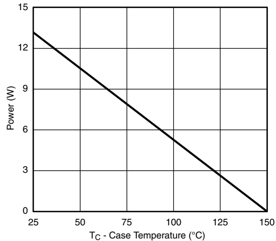
Power Derating
