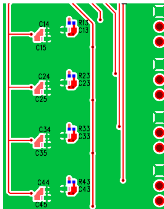
Figure 1. Hybrid Control Resistors
