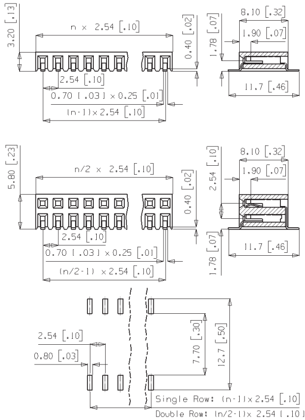
PCB Layout
