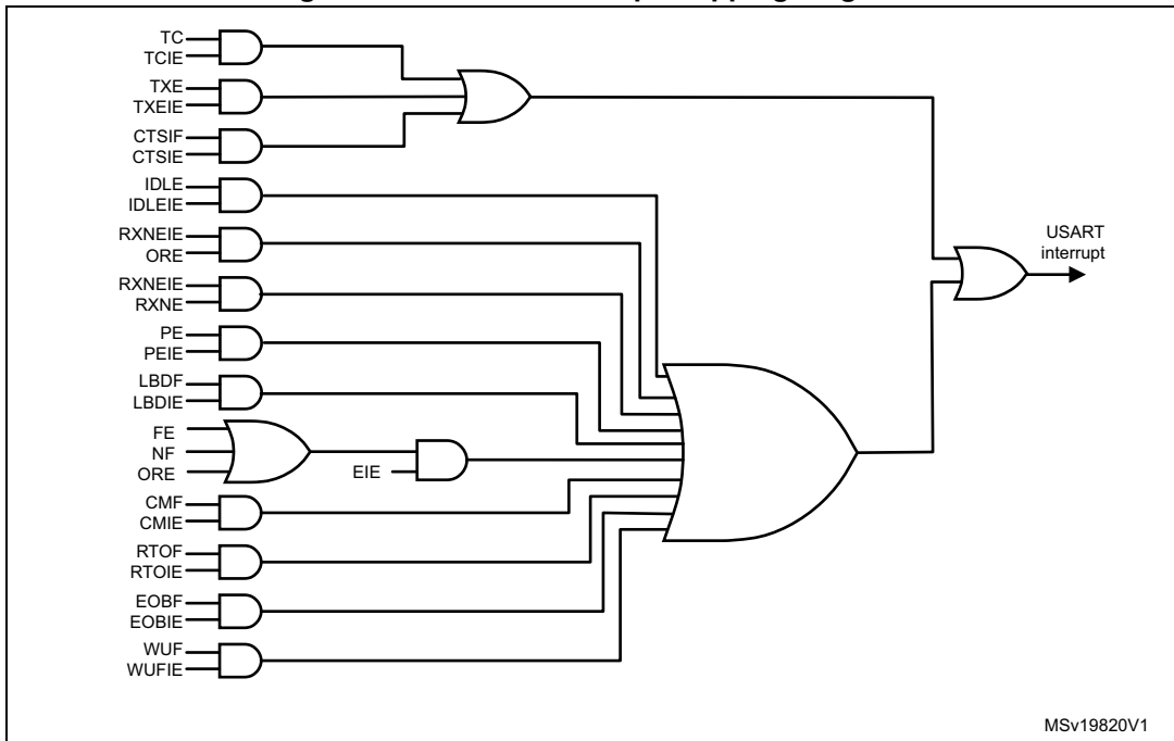
Figure 259. USART interrupt mapping diagram
