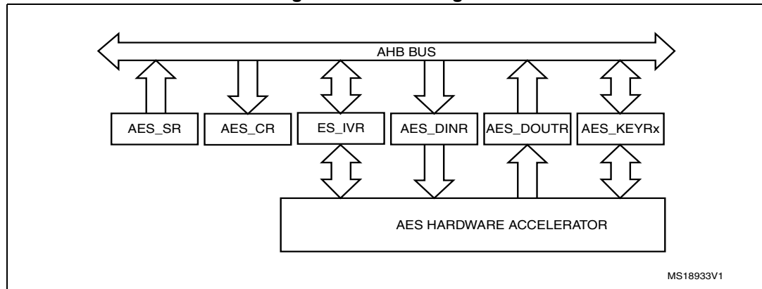
Figure 79. Block diagram
