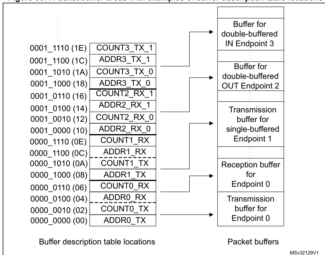
Figure 307. Packet buffer areas with examples of buffer description table locations
