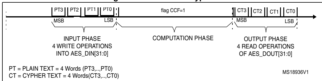
Figure 90. Mode 1: encryption
