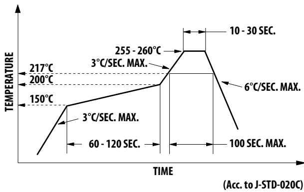
Figure 15. Recommended Reflow Soldering Profile
